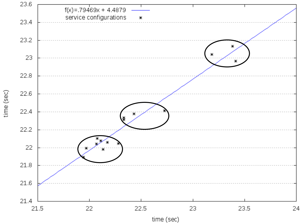
Figure 2. 4GB “m-bound” regression plot (XEN)
